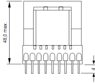
Dimensions [mm]
